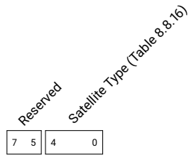
Field 8.8.8: Additional satellite information ( sat_info )
