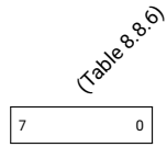
Field 8.8.3: Signal constellation, band and code ( sid.code )
