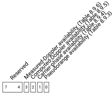
Field 8.9.2: Observation availability at filter update ( sv_tel[N].availability_flags )
